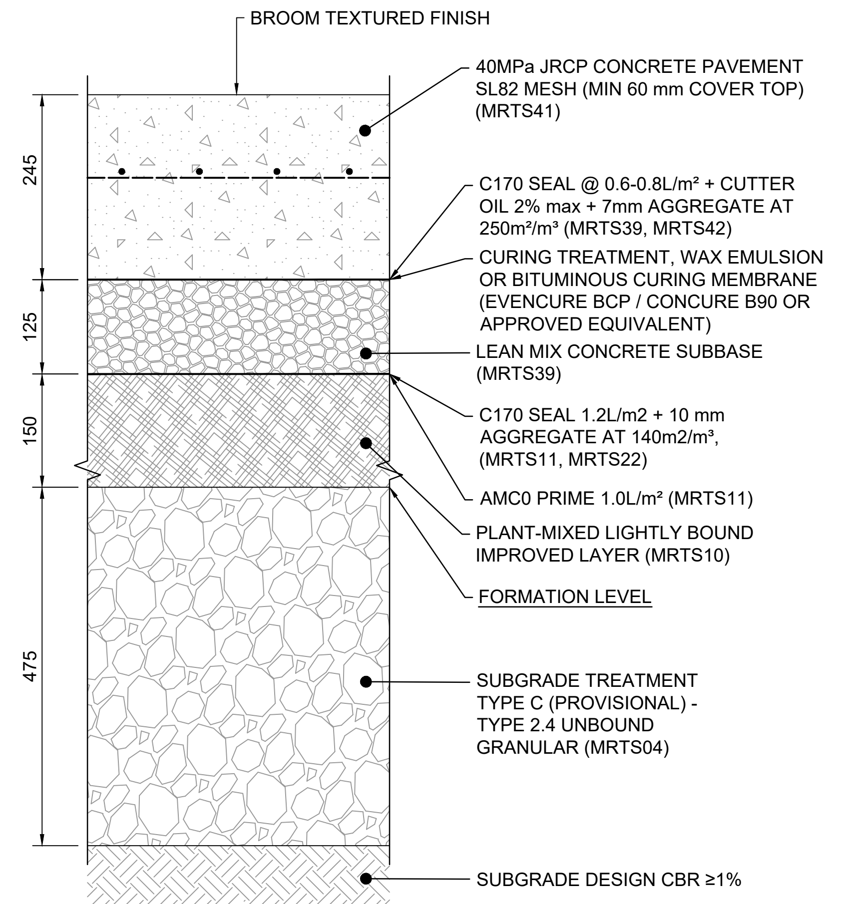
RP1 - JOINTED REINFORCED CONCRETE PAVEMENT (JRCP)
