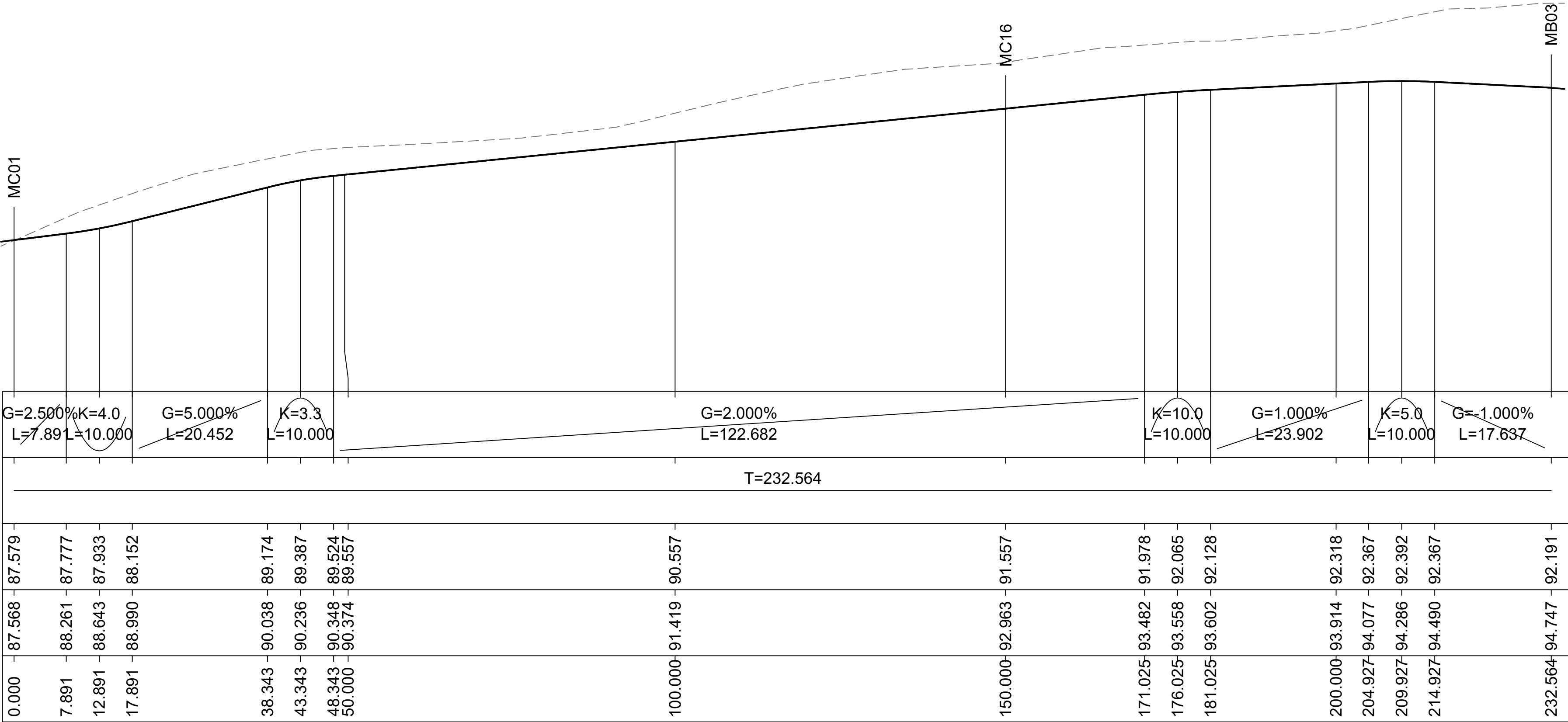
LONGITUDINAL SECTION OF MC15 CONTROL LINE
