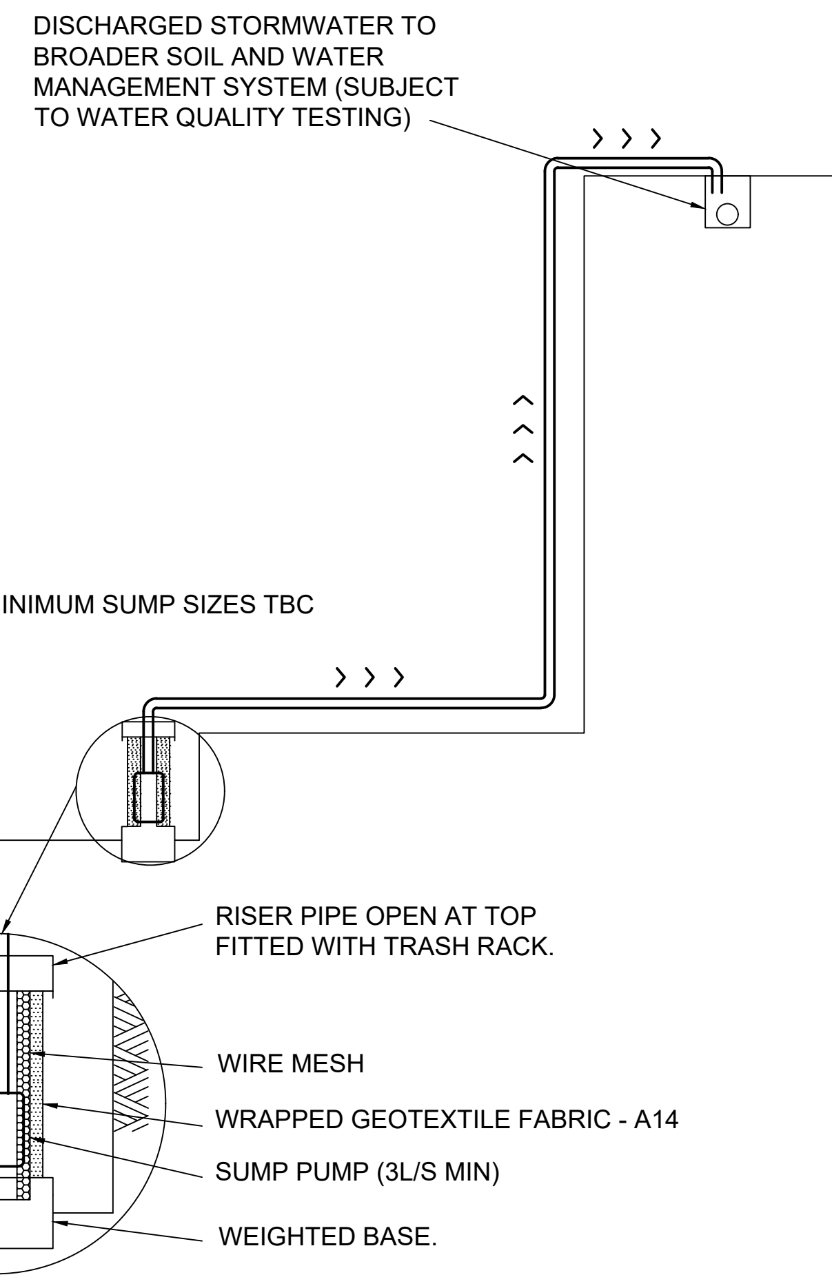
STORMWATER SUMP AND OUTLET
